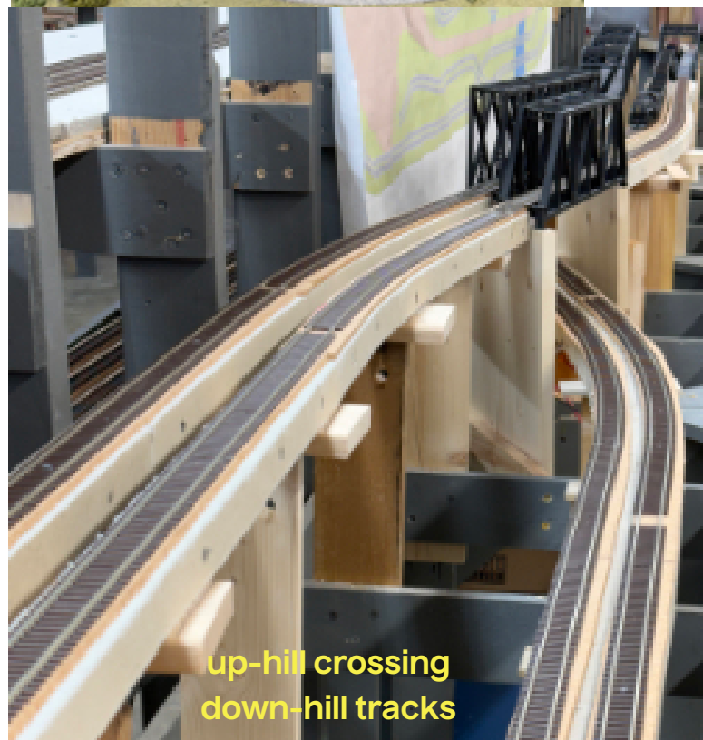
COMRC Modular Layout
